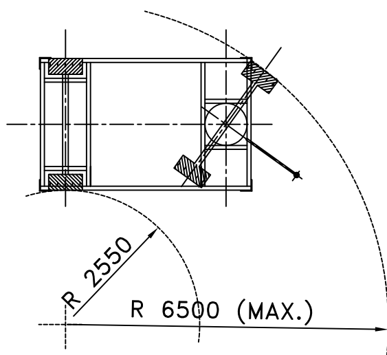
TURNING RADIUS DETAIL
