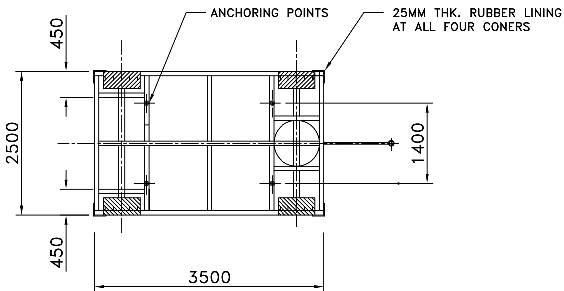
CHANNEL STRUCTURE PLAN
